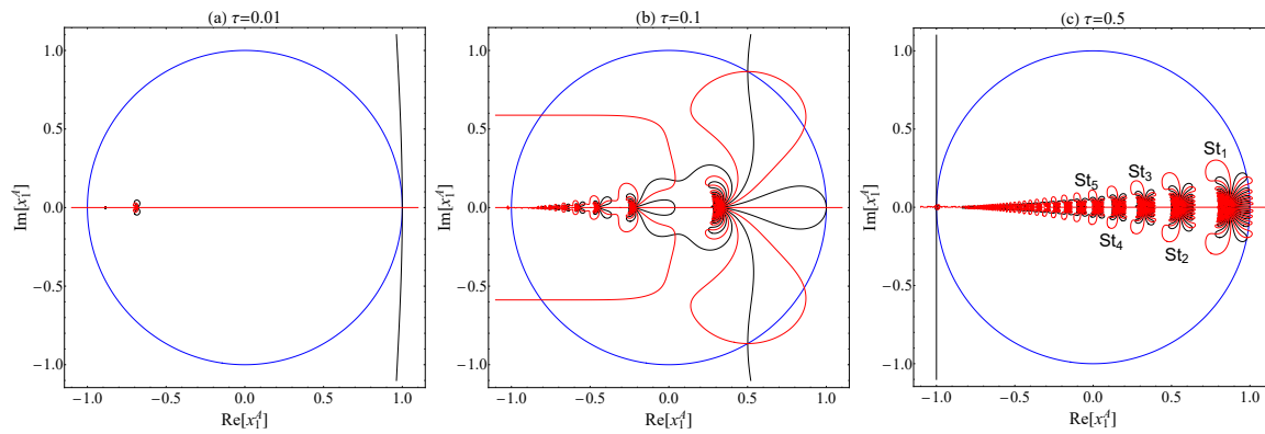
FIG. 2. Contour plots of f(x_1^A) in the x_1^A -complex plane. Black lines refer to the curve where \text{Re}[f(x_1^A)] = 0 , while the red ones refer to \text{Im}[f(x_1^A)] = 0 . The blue curve represents the unitary circle. Solutions of Eq. (46) are given by the intersections of black and red lines. In panels (a)-(c), the value of \tau was chosen to be 0.01, 0.1, and 0.5, respectively. The other numerical parameters are shown in Eq. (43). A magnification of structures \text{St}_1, \dots, \text{St}_4 , seen in panel (c), is shown in Fig. 3.
