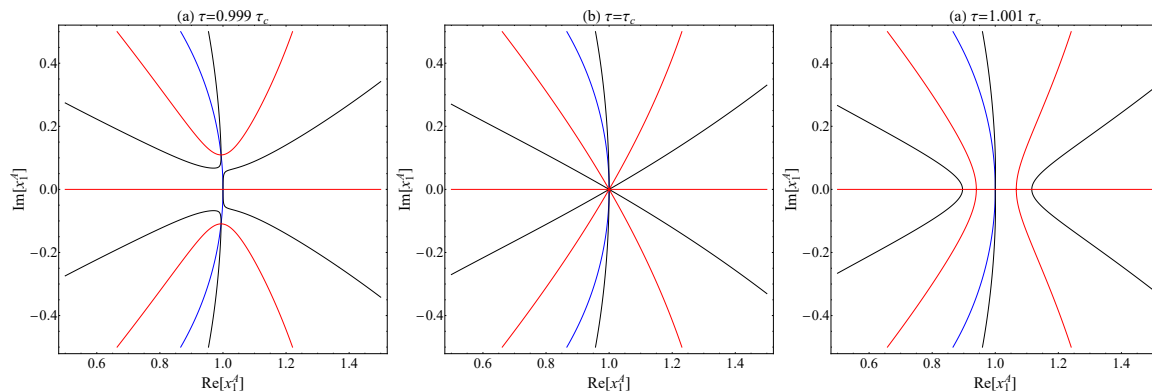
FIG. 5. The same as Fig. 2, but with imaginary dimensionless time: (a) \tau = 0.999\tau_c , (b) \tau = \tau_c , and (c) \tau = 1.001\tau_c .
