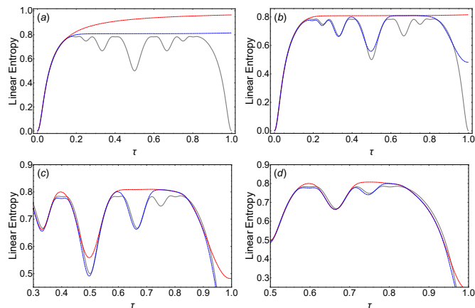
FIG. 4. Linear entropy as a function of \tau . In panel (a), the red dashed curve represents the semiclassical entropy exclusively based on real trajectories, while the blue dotted line shows the result of Eq. (27) when the roots marked in Fig. 3(a) are used. This result, for comparison purposes, is reproduced as the red dashed line in panel (b), where the blue dotted line represents S_{sc} , improved by the inclusion of the roots marked in Fig. 3(b). The same logic is applied to panels (c) and (d), where the red dashed curve is copied from the previous plot, and the blue dotted curve shows the result of S_{sc} when the roots of Figs. 3(c) and 3(d), respectively, are included. The gray solid line appearing in all panels shows the quantum entropy (42). The numerical parameters used here are shown in Eq. (43).
