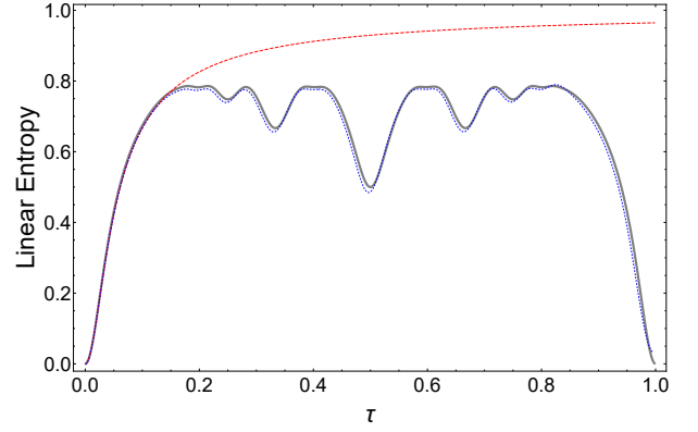
FIG. 1. The gray solid line illustrates the quantum linear entropy (42) as a function of the dimensionless time \tau . We also show results for the semiclassical entropy (27): the red dashed line illustrates S_{sc} when we take into account only real trajectories, while the blue dotted line contemplates the inclusion of a few dozens of complex sets. The numerical parameters used to build this figure are given by Eq. (43).
