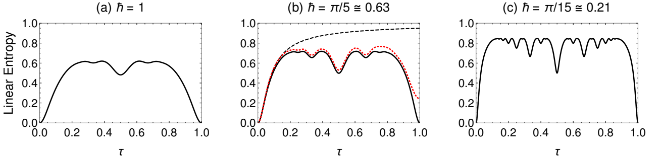
FIG. 1. Black solid lines represent quantum linear entropy of the reduced state (39) as function of the dimensionless time \tau , for (a) \hbar = 1 , (b) \hbar = \pi/5 , and (c) \hbar = \pi/15 . Other numerical parameters are E_{0r} = \omega_{0r} = \lambda = 1 and z_{0r} = \sqrt{E_{0r}/(\hbar\omega_r)} . In panel (b), the black dashed curve shows the contribution of the set of real trajectories to \mathcal{S}_{\text{lin}} , while the red dotted one presents the equivalent result when a few sets of complex trajectories are considered.
