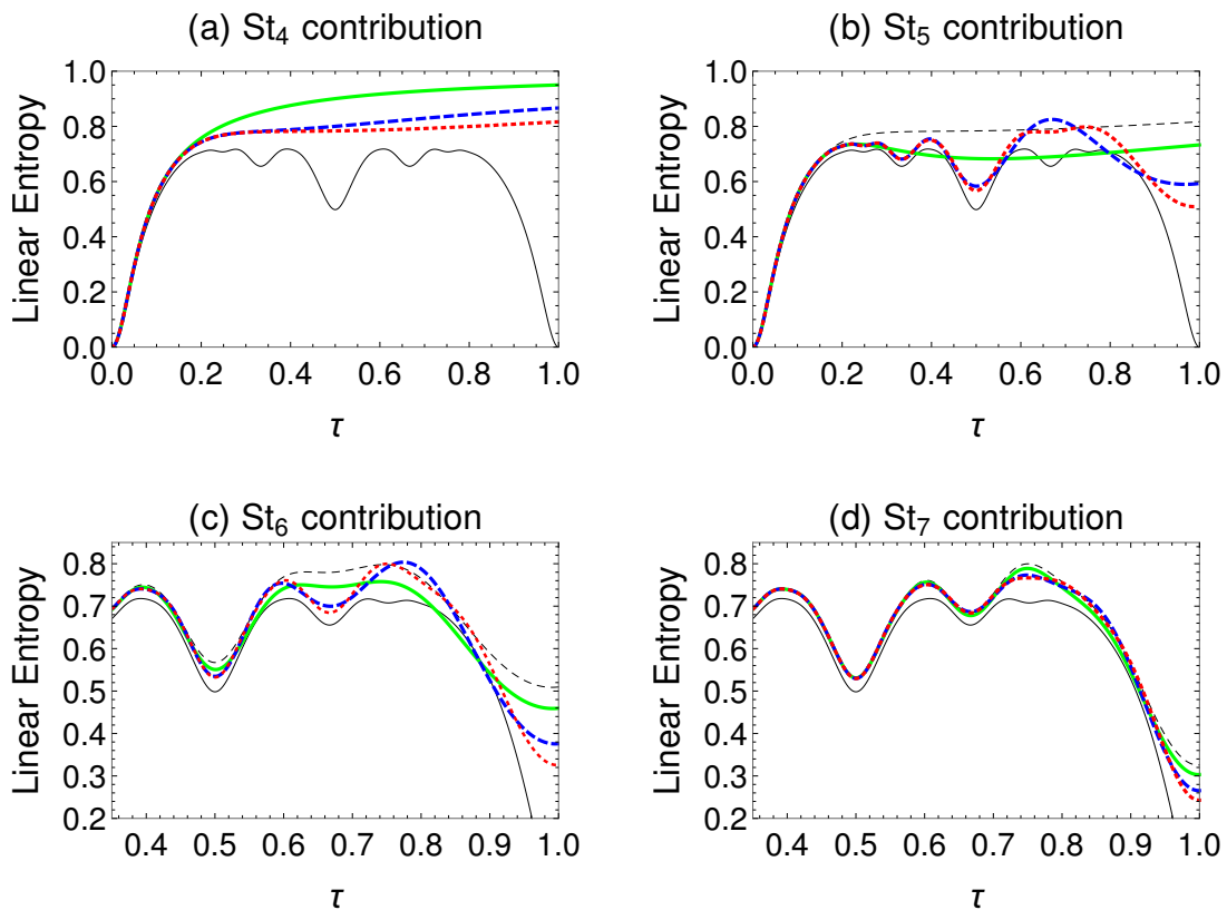
FIG. 3. Black solid lines represent the quantum linear entropy of the reduced state (39) as function of the dimensionless time \tau . Numerical parameters are chosen to be the same of those of Fig. 1(b). In panel (a), the solid green line refers to \mathcal{S}_{\text{lin}} , calculated using exclusively the set of real trajectories, associated with the root inside the green circle of Fig. 2(i); including trajectories associated with the root marked by the blue circle of Fig. 2(i) produces the blue dashed curve; and, including contributions related to the root marked by the red circle of Fig. 2(i) generates the red dotted curve. Colored lines of panels (b), (c), and (d) are built analogously to panel (a); by adding contributions to the semiclassical approach presented in Fig. 2(j), Fig. 2(k), and Fig. 2(l), respectively. Black dashed lines in panels (b), (c), and (d) are the most complete curve of the preceding panel, i.e., the red dotted curve of panels (a), (b), and (c), respectively.
