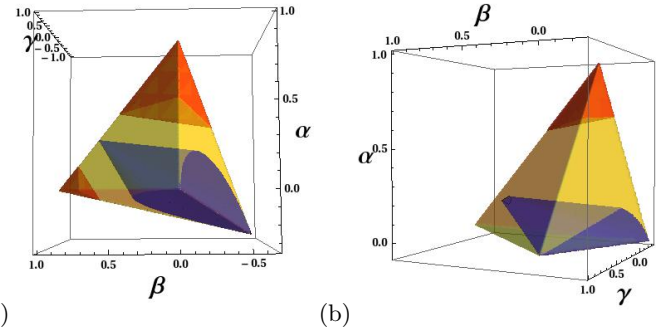
FIG. 1. Geometrical representation of states \rho_{\alpha,\beta,\gamma} [Eq. (37)] in parameter space for (a) 2j + 1 = 3 and (b) 2j + 1 = 5 . All physical states lie inside the tetrahedron whereas the PPT states lie inside the blue region [a cone for the 2-qudit case (a)]. Red regions depict entangled states detected using our criterion Eq. (15), whereas the yellow region hosts the non detected entangled states by this criterion.
